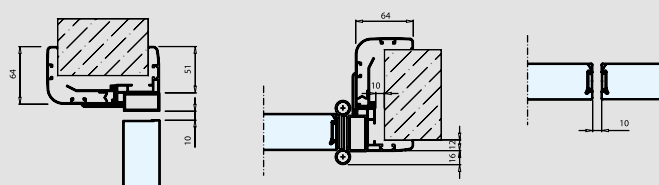
Section opening swing leaf with embracing frame.
