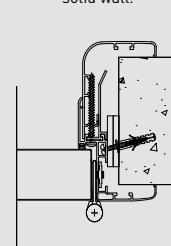
Fixing on solid wall.
