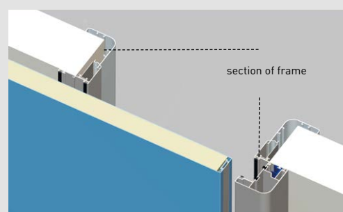
Section of sliding leaf outside wall.
