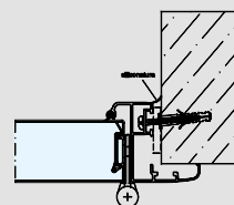
Fixing on solid wall.
