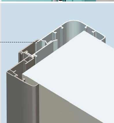
Fixing on gypsum carton wall.
