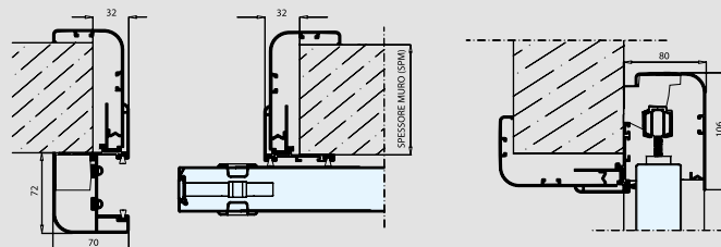
Section of sliding leaf outside wall.
