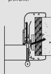
Fixing on wooden preframe.
