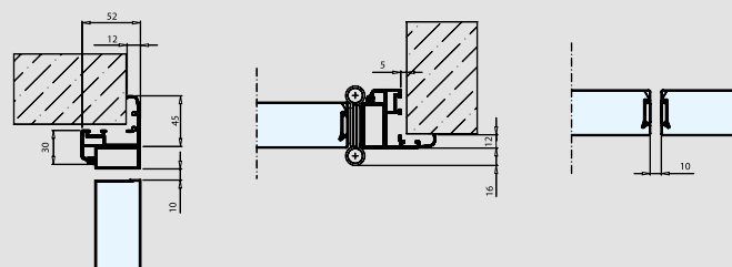
Section opening swing leaf with corner frame.
