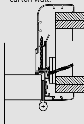
Fixing on gypsum carton wall.
