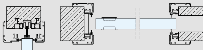
Section sliding opening leaf inside wall.
