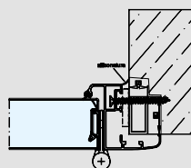
Fixing on wooden preframe.
