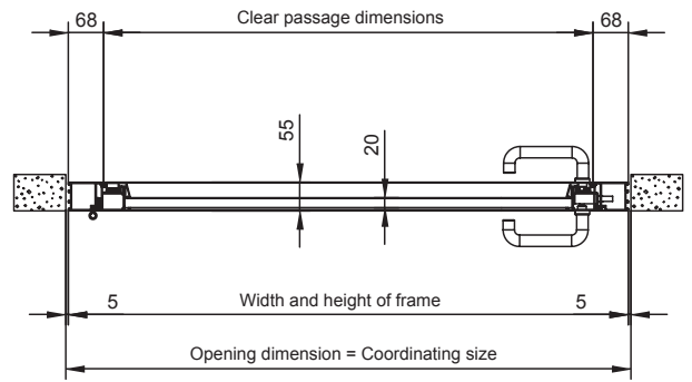
Horizontal section/ Installation in the opening
