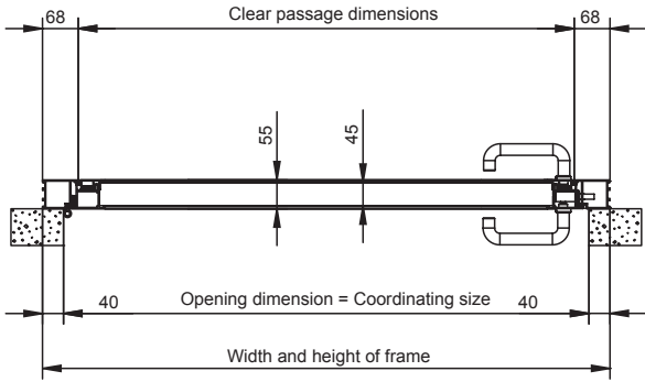
Horizontal section/ Installation behind the opening
